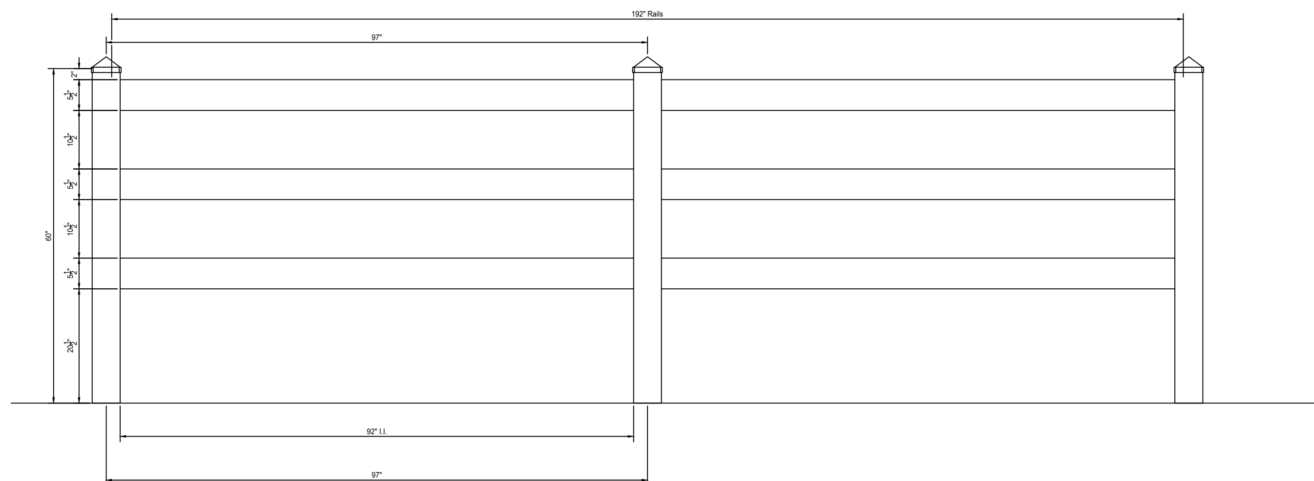
ELEVATION VIEW
